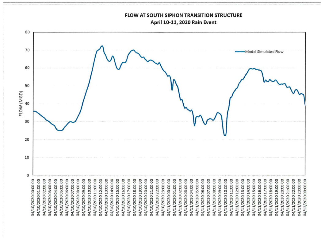
Figure 3. Flows at South Siphon Transition Structure (estimated)
