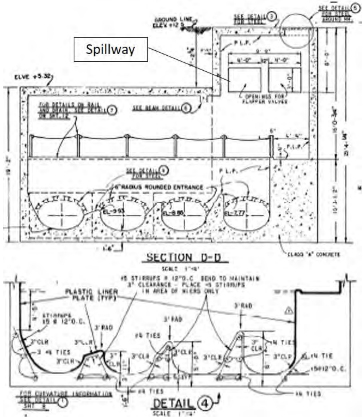
Figure 3. Sweetwater River Crossing Siphon
