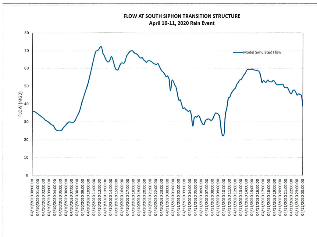
Figure 3. Flows at South Siphon Transition Structure (estimated)
