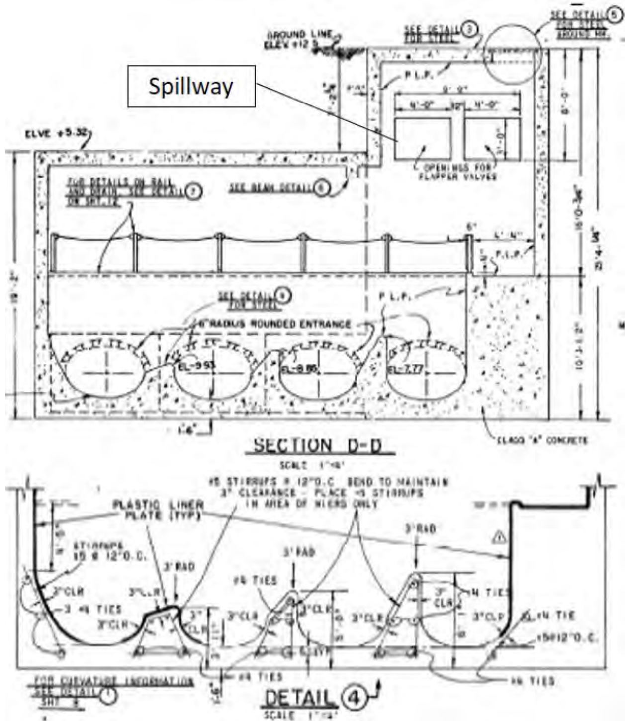
Figure 3. Sweetwater River Crossing Siphon
