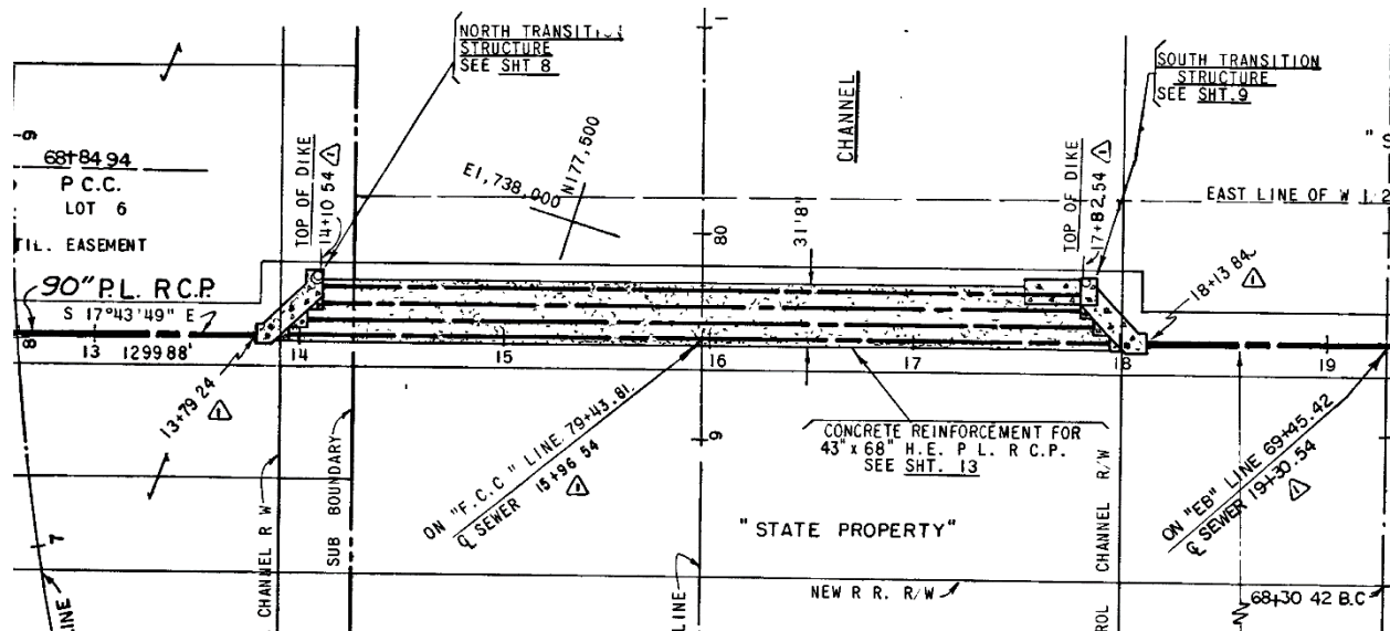
Figure 1. Sweetwater River Crossing Siphon
