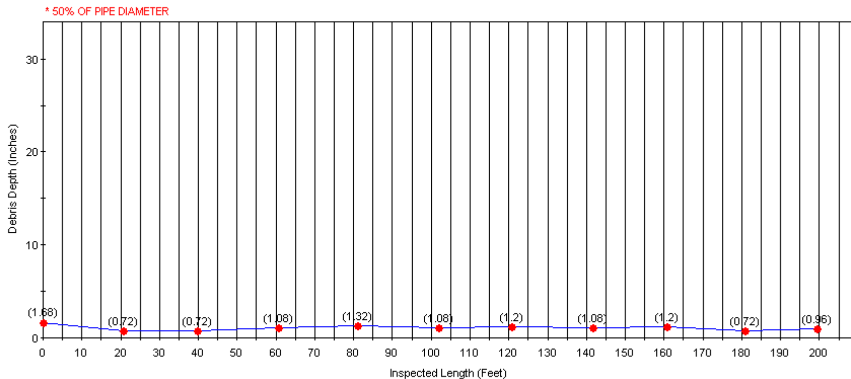
Sonar Inspection Profile
