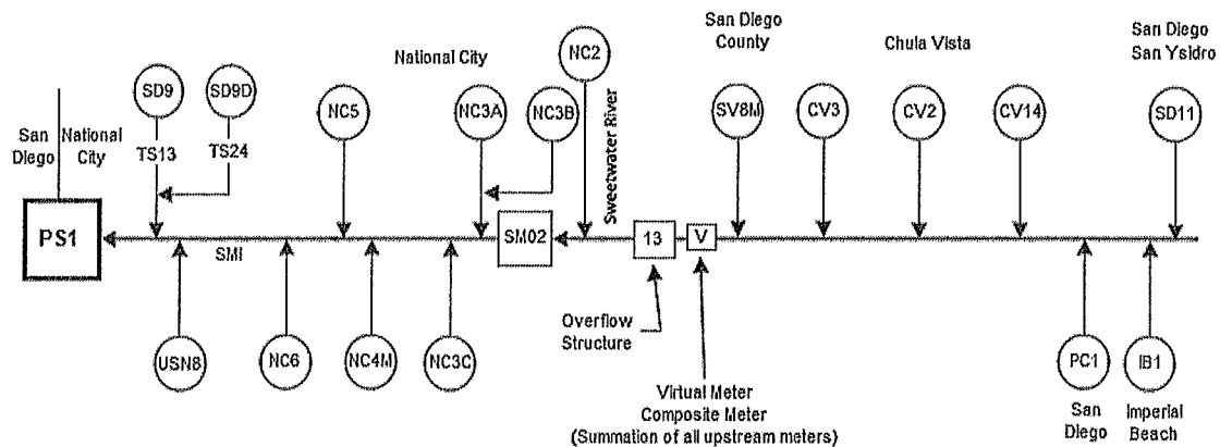
Figure 1. Tier-one Wastewater Flow Meters and Their Locations Relative to PS1 and Each Other
