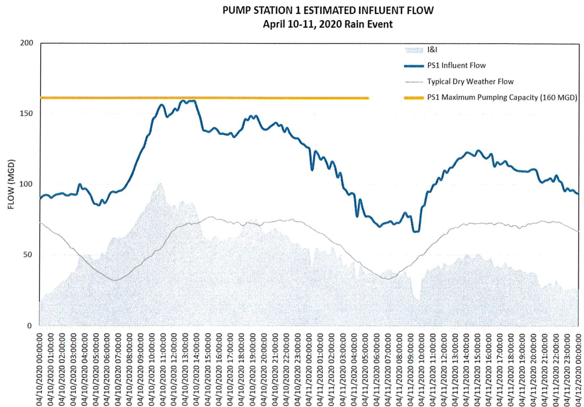
Figure 2. PS1 Influent Flow on April 10-11, 2020
