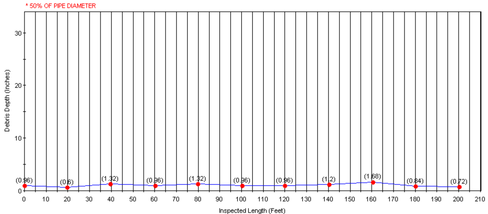
Sonar Inspection Profile
